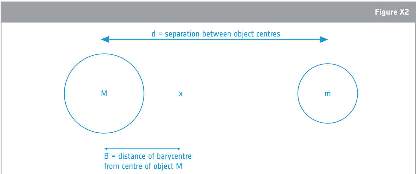
↑ Two objects (mass M and m ) in orbit about a common centre of mass or barycentre. The objects are separated by a distance d and the distance between the centre of the most massive object M and the barycentre is B .
